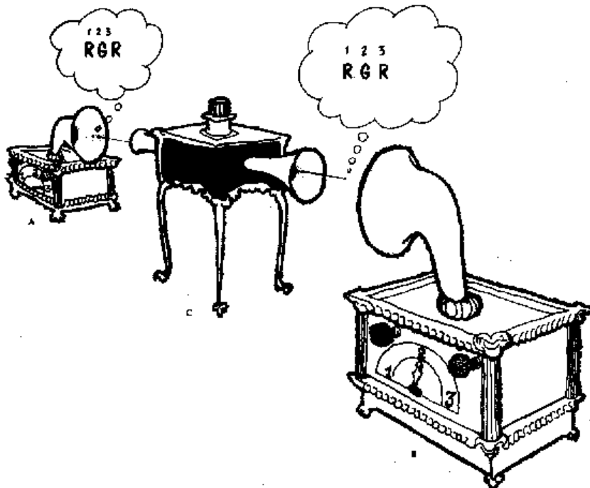
Figure 7 – Instruction sets.
