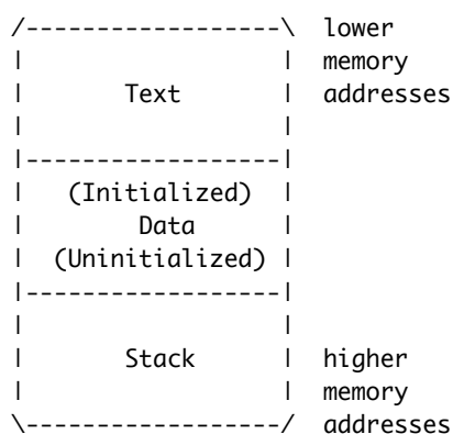
Fig. 1 Process Memory Regions
